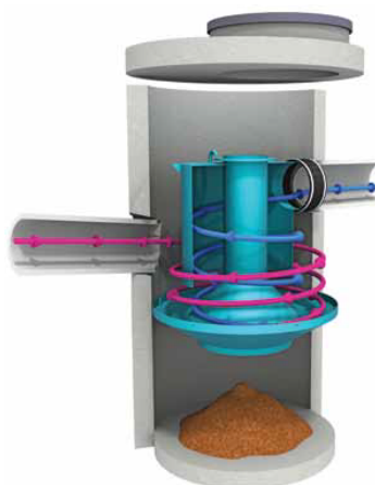
Figure 1 – Schematic of the Downstream Defender® Oil Grit Separator
